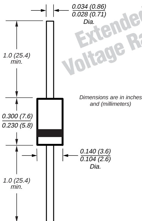
DO-204AC (DO-15)
